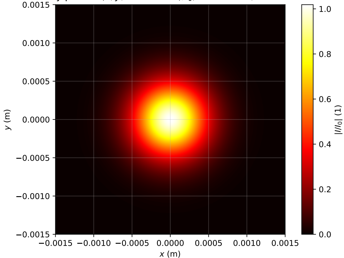
Intensity profile I(x, y, z = 0.716m)/I_0 , Pin=0.4Pcr, artificial time
